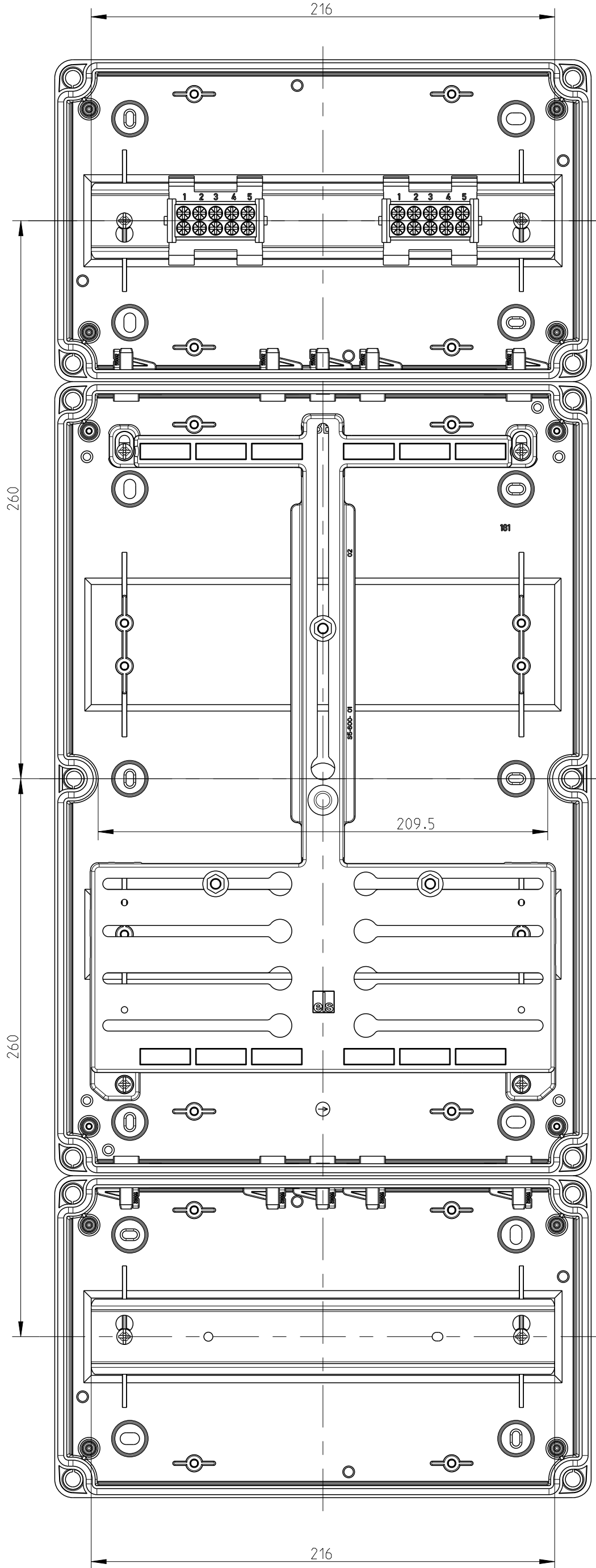
1:5 Innenansicht interior view ZKi 110 ZKi 110-f
